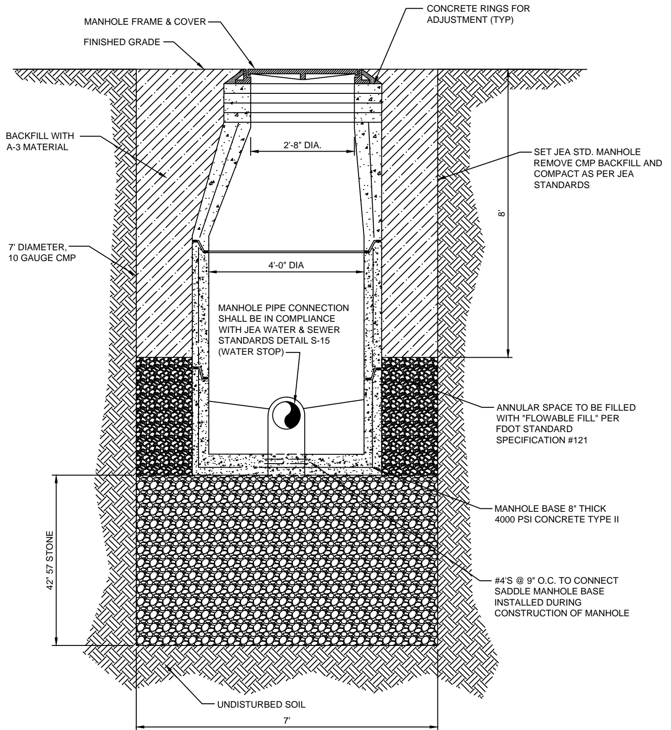
SECTION VIEW
