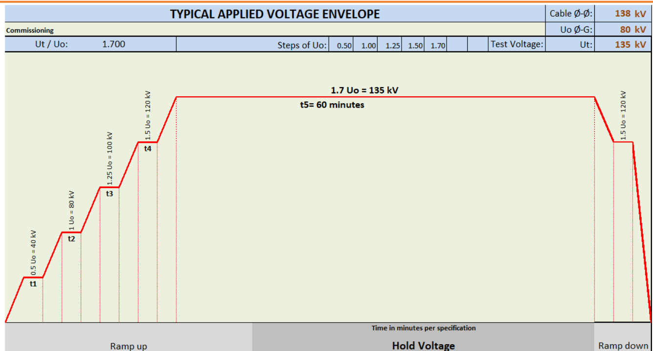
Figure 2: Typical Voltage Envelope
