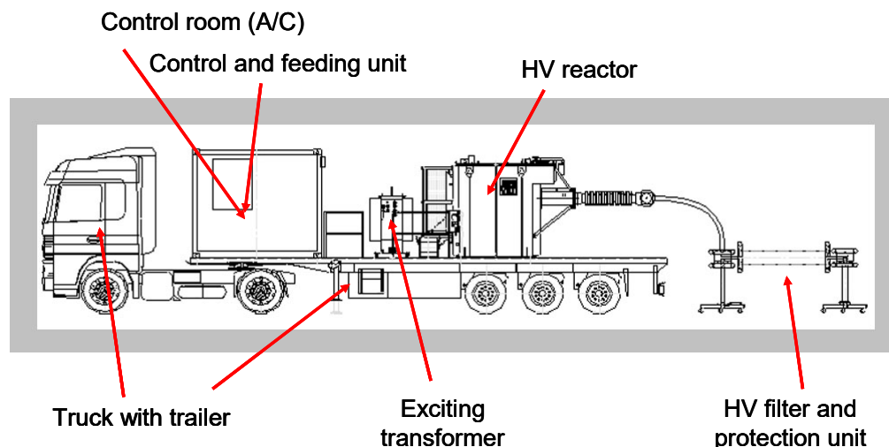
Figure 1: Sketch of one mobile RTS system.
