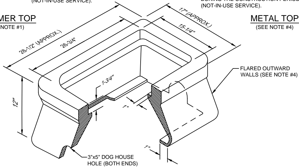
POLYMER BOX
